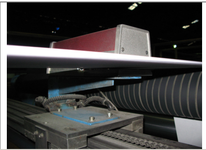
Model 1088 Sentinel® Splice Detector™ Jagenberg Sheeter
